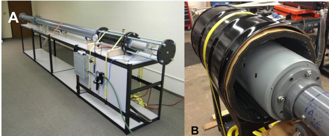
Figure 4.1: (A) High impulse blast tube. (B) Silencer attachment for noise reduction.
