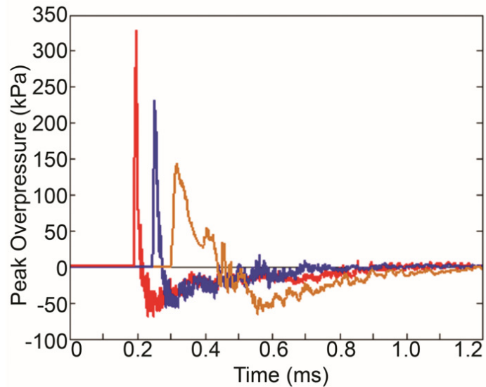
Figure 2.1: Representative pressure traces at the three test locations measured in air. Peak pressure values are 323, 232, and 145 kPa. The traces are offset to clearly display each waveform. Sampling at 2.5 MHz was confirmed to be sufficient by comparison to redundant sampling with a digital oscilloscope at 2 GHz.
